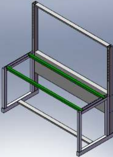
Discovery LT™ "H" leg single sided assembly with 76" h slotted uprights
