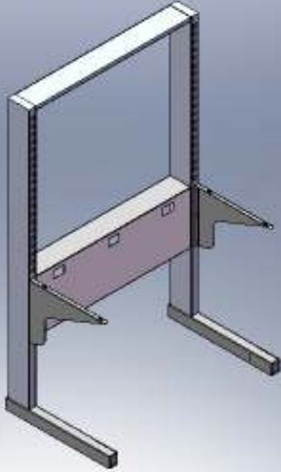
Single sided Discovery™ bench full height module 82"
