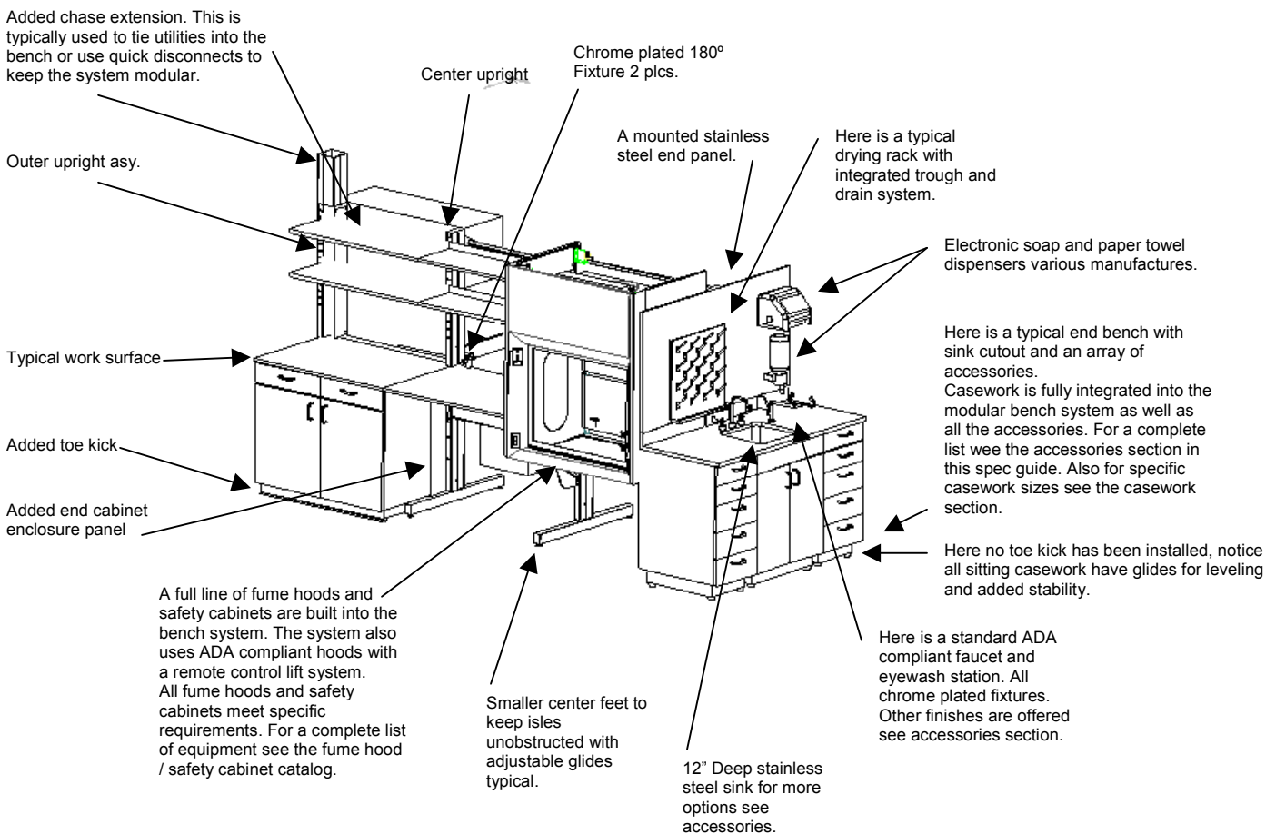
FIGURE 3. Complete Discovery Bench Layout Side A
