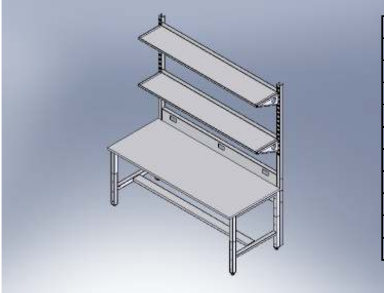
EKO Bench with full height uprights, power bridge assembly, and flat shelves
